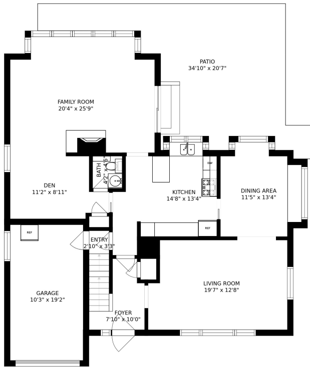
FIRST FLOOR 127 RIVERSIDE DR, NORTHFIELD, IL 60093
