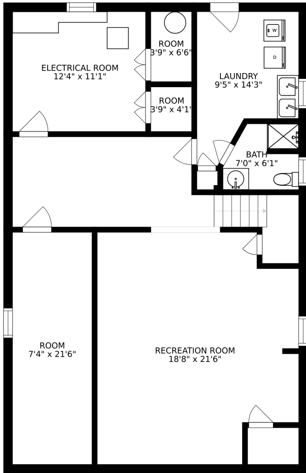
FLOOR 1
