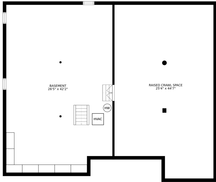
BASEMENT
