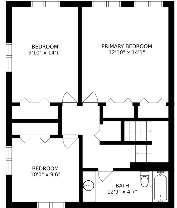
FLOOR 3
