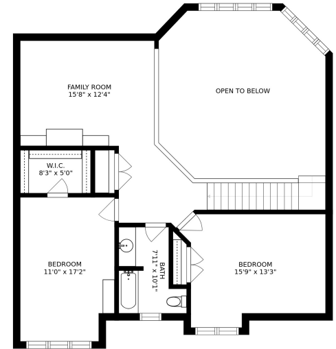
FLOOR 3
