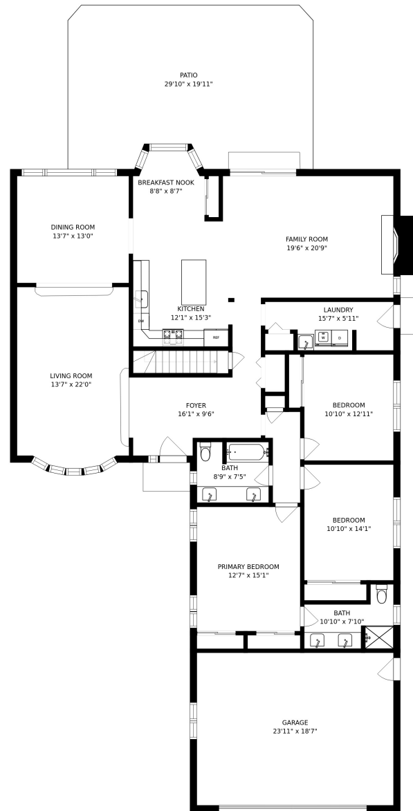
FLOOR 2
