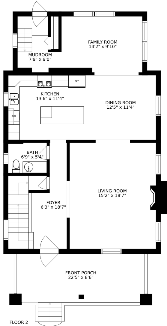
FLOOR 2
