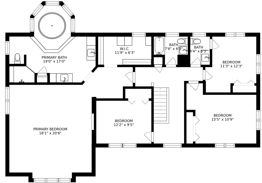
FLOOR 3
