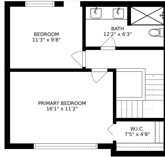
FLOOR 3
