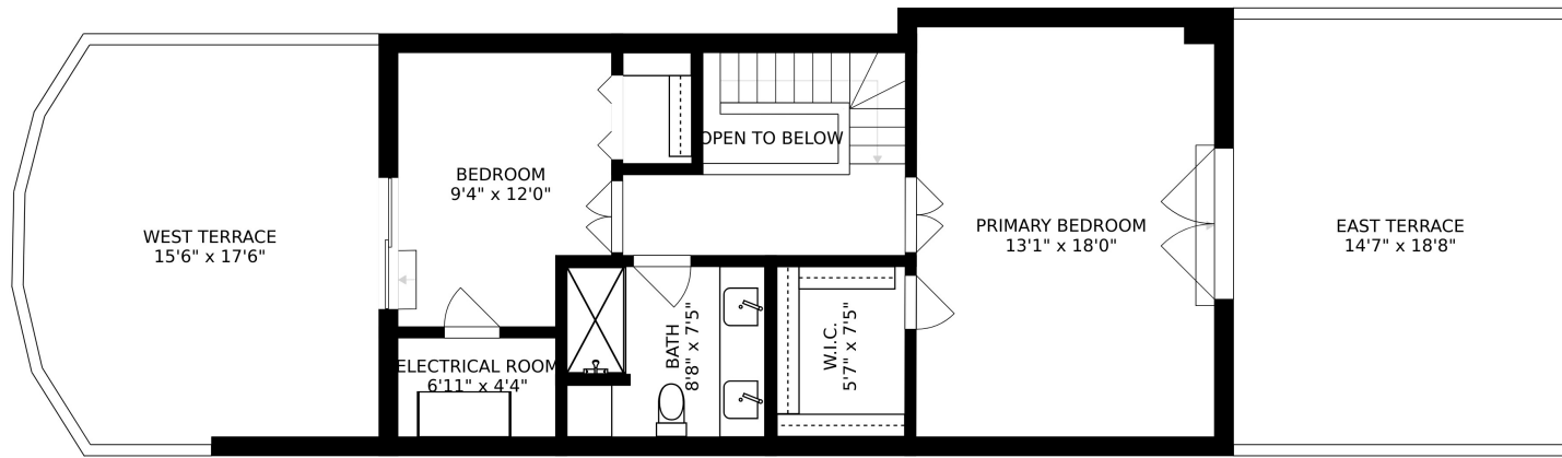
FLOOR 3
