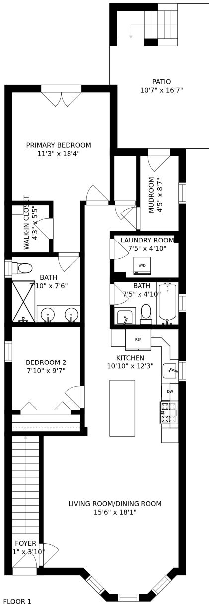
FLOOR 1
