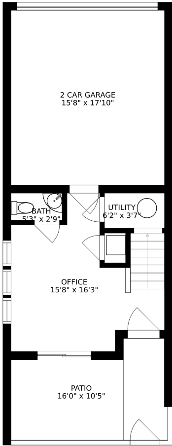
FLOOR 1
