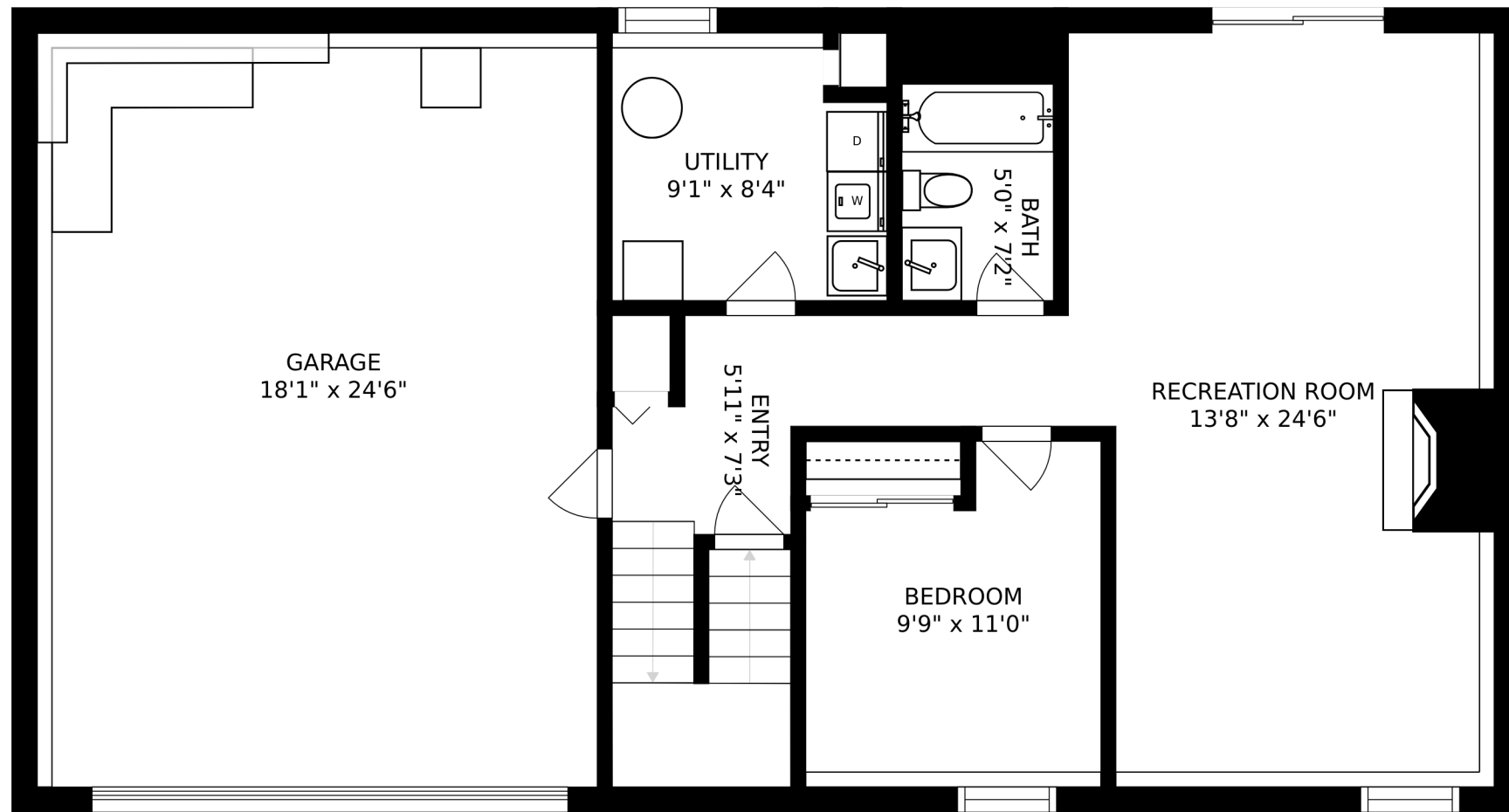
FLOOR 1
