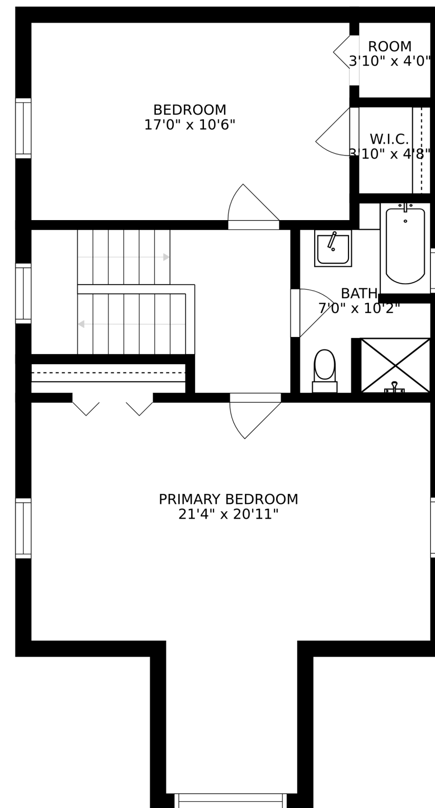
FLOOR 3
