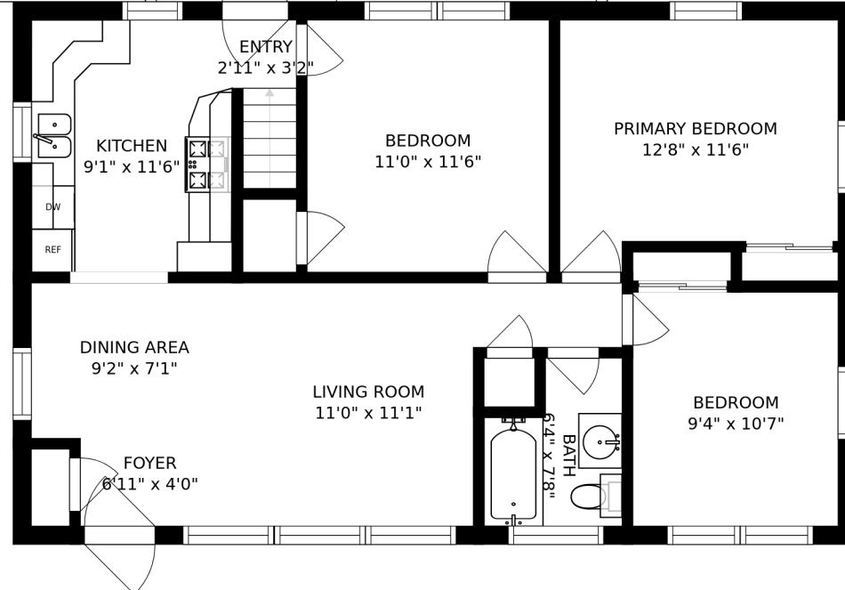
FLOOR 2
