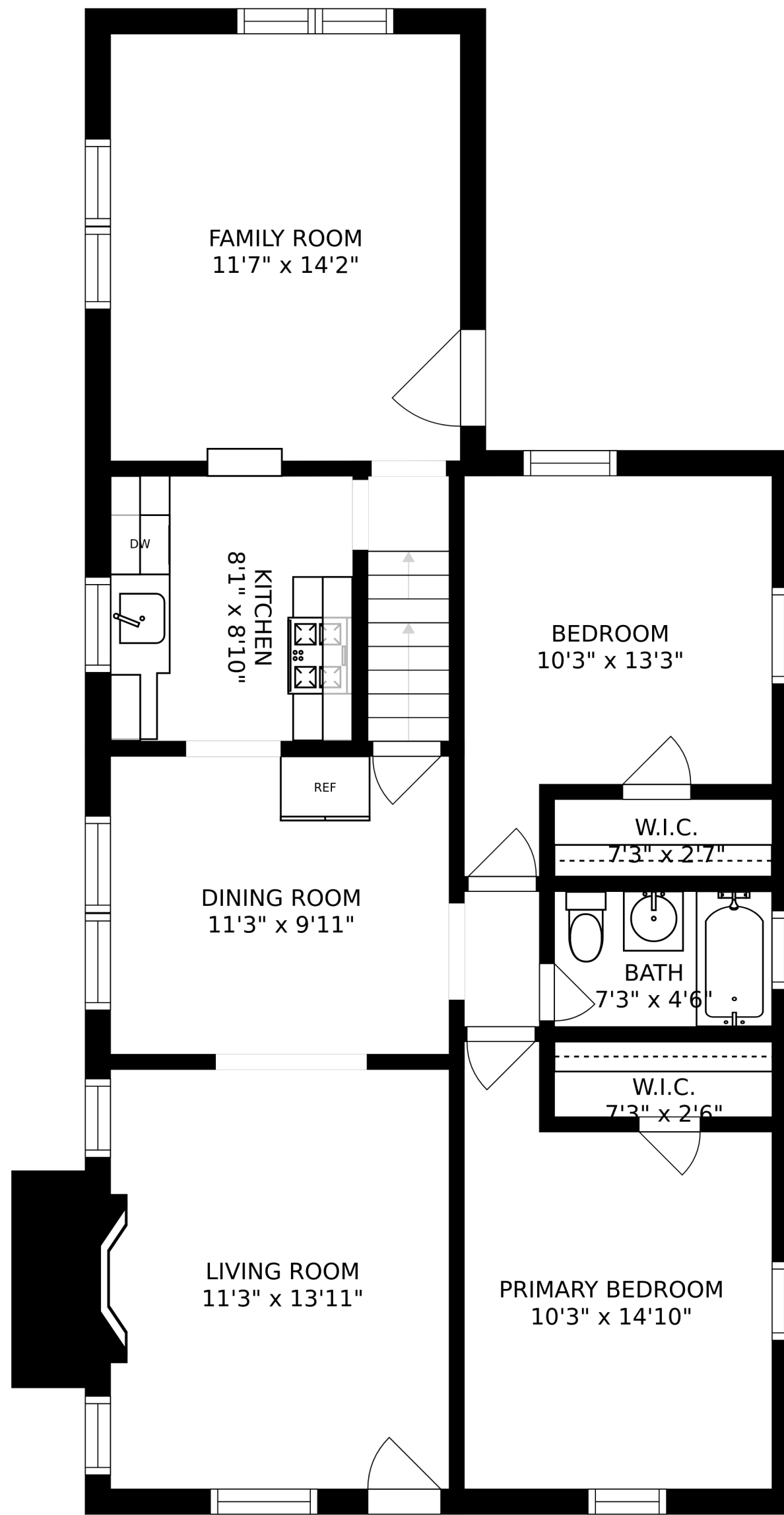
FLOOR 2
