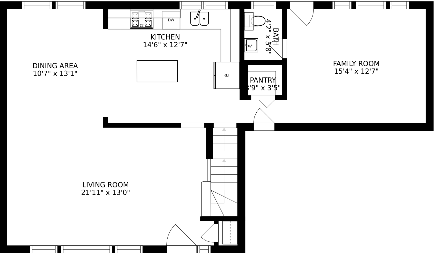
FLOOR 2
