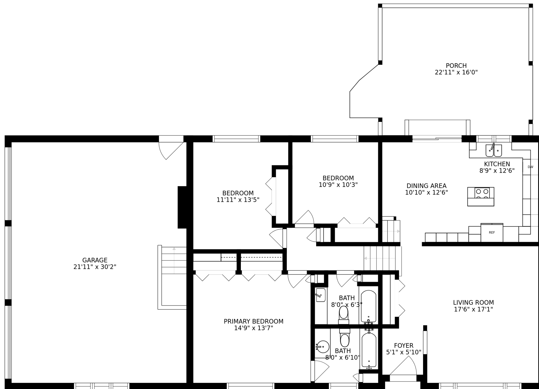
FLOOR 2
