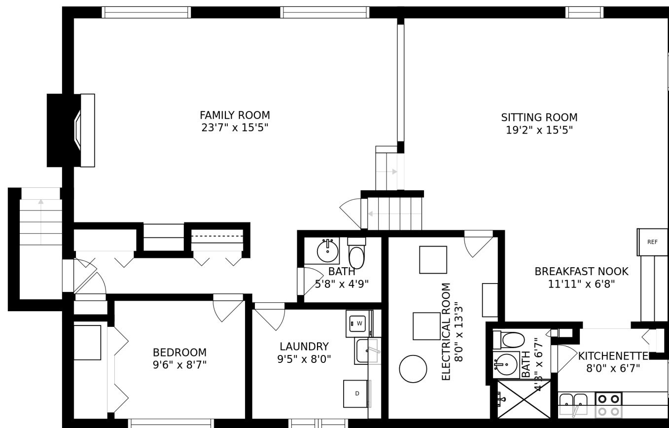
FLOOR 1
