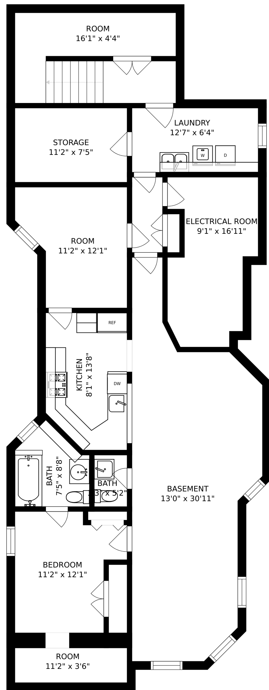
FLOOR 1
