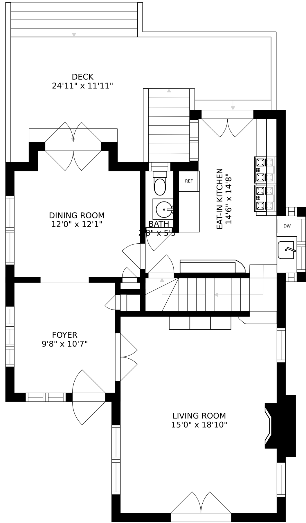
FLOOR 2
