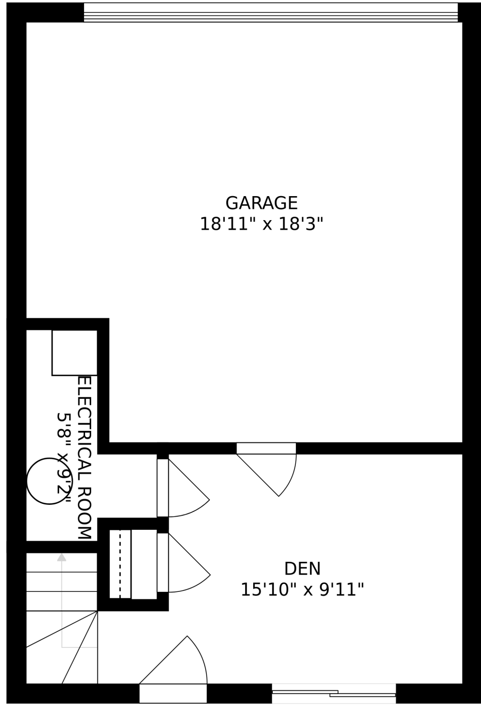
FLOOR 1
