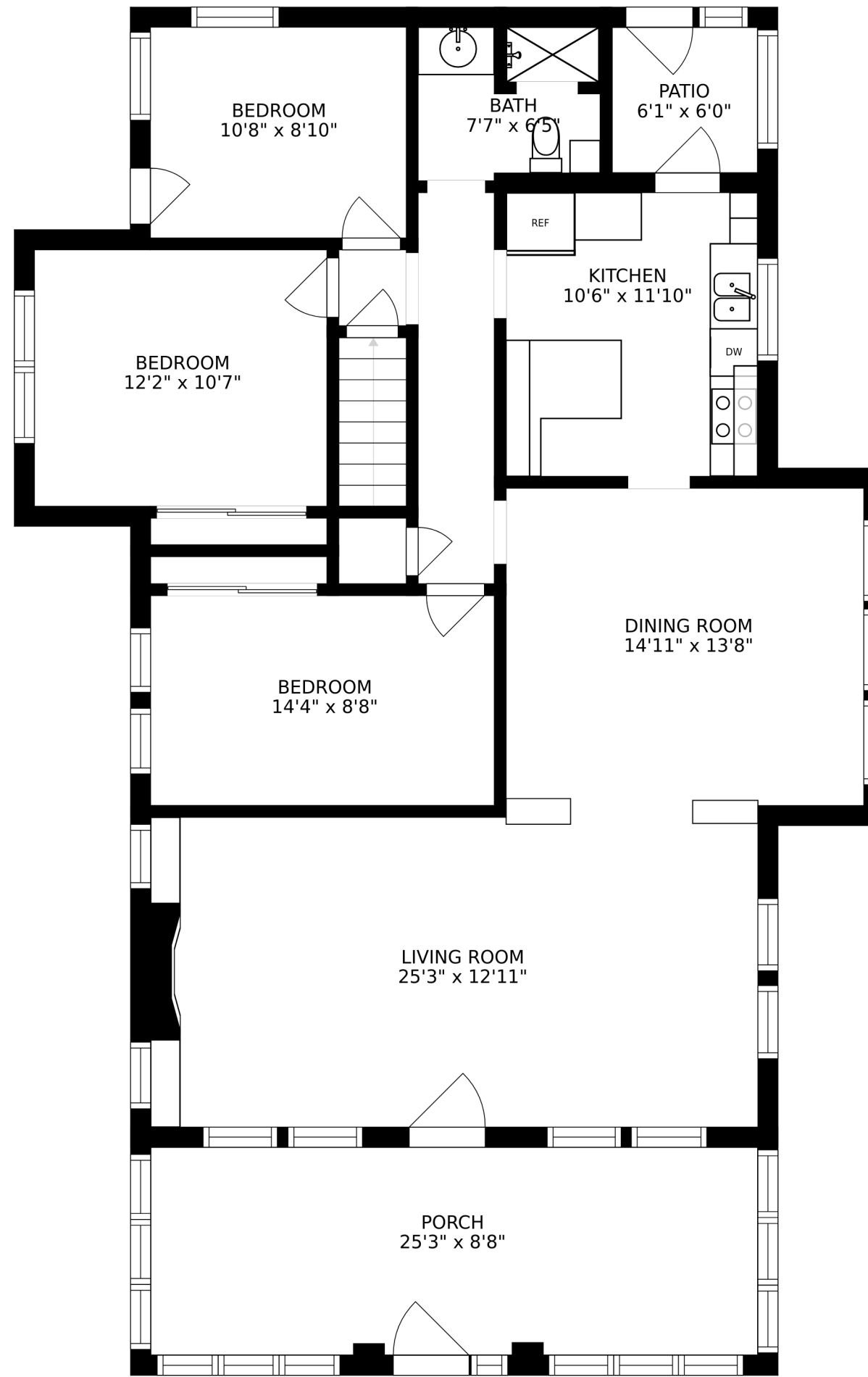
FLOOR 2
