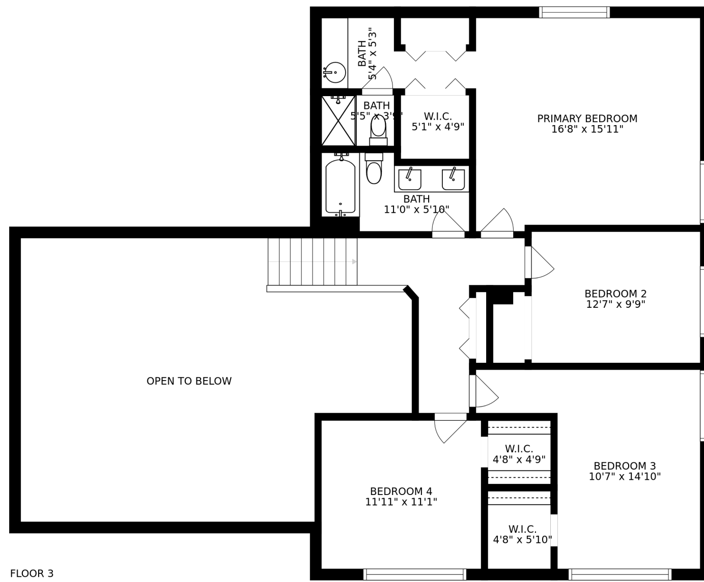
FLOOR 3
