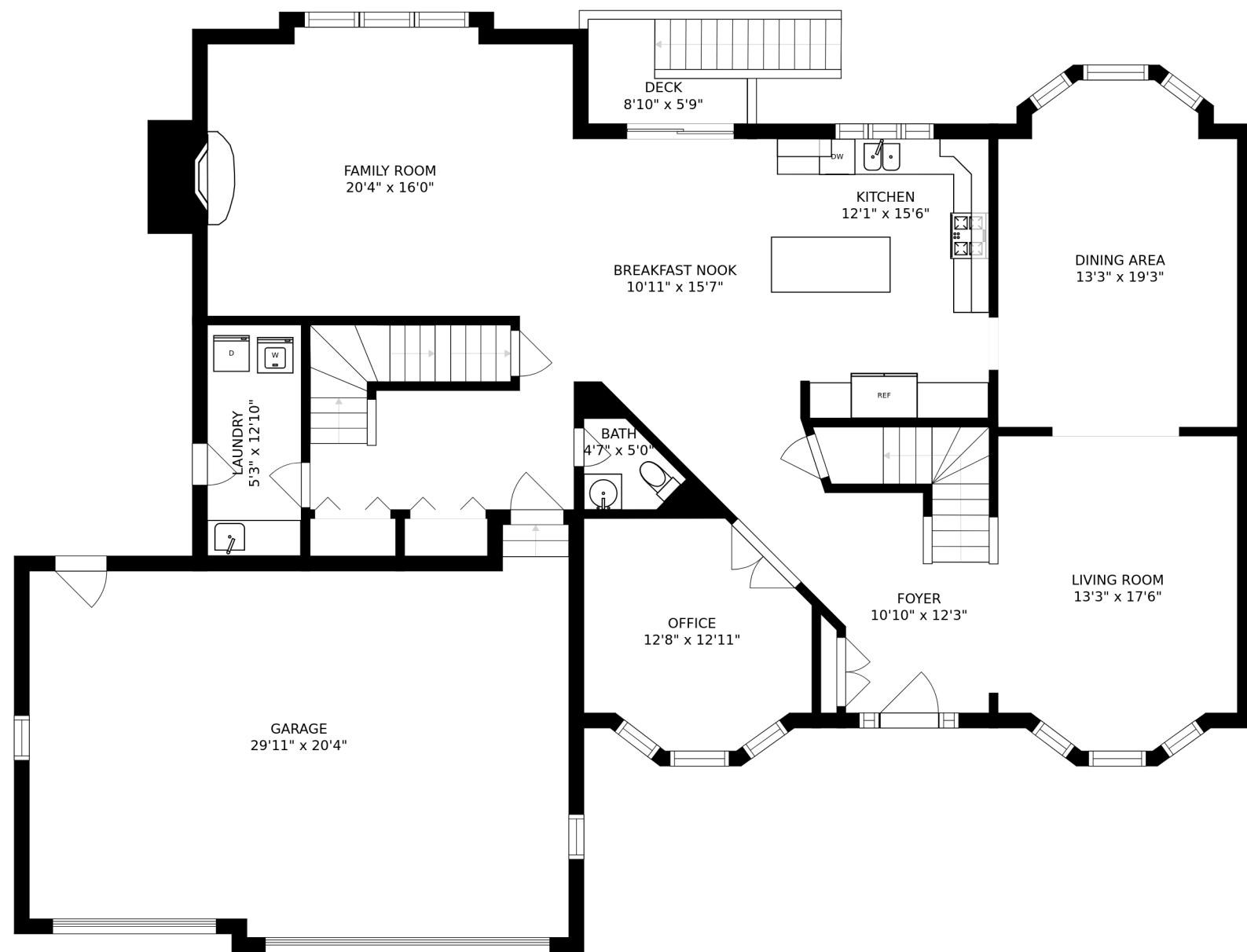
FLOOR 2
