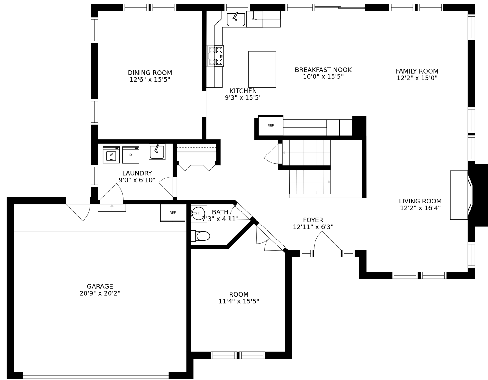
FLOOR 2
