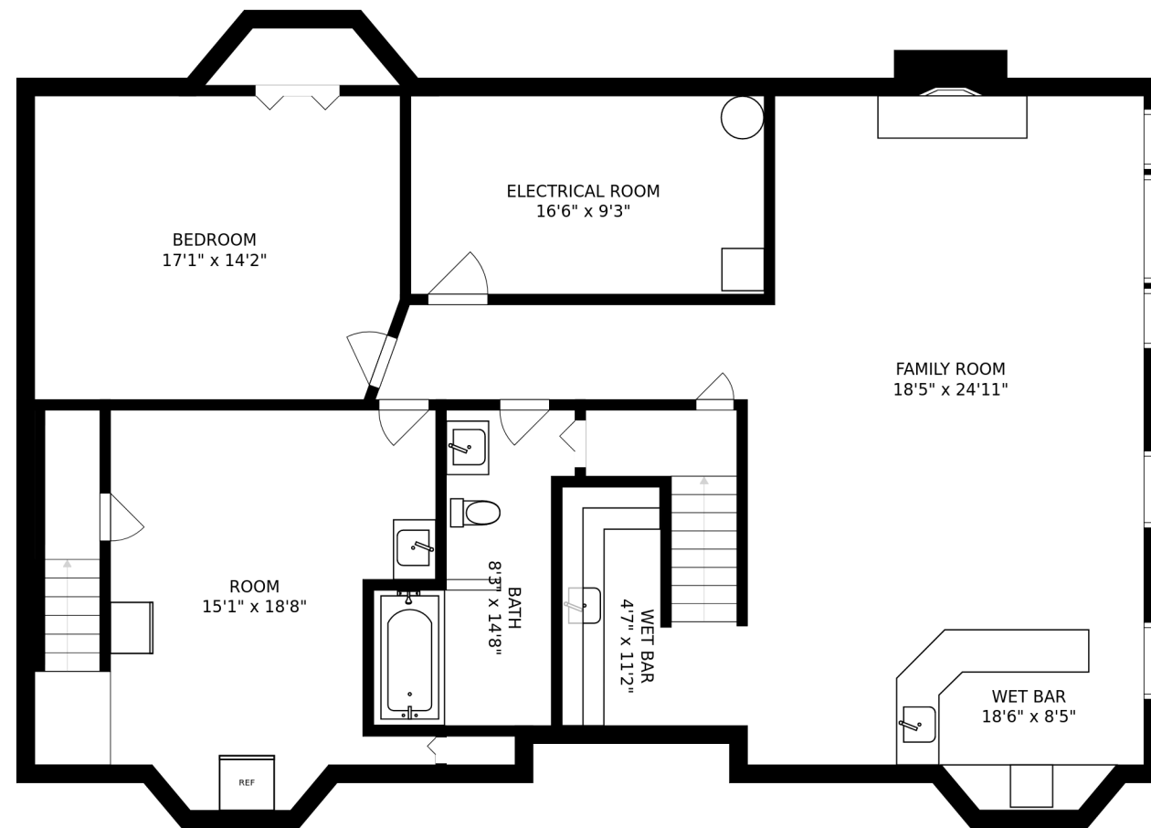
FLOOR 1
