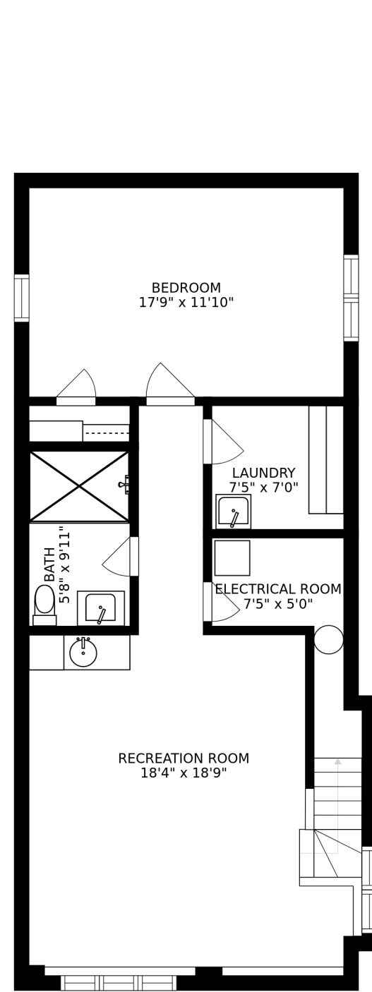
FLOOR 1
