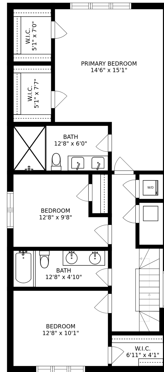
FLOOR 3
