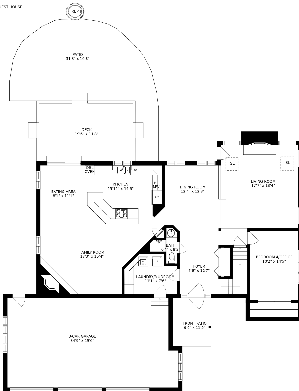
FLOOR 1
