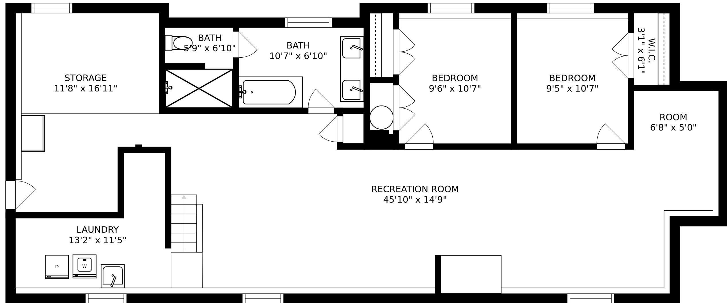
FLOOR 1
