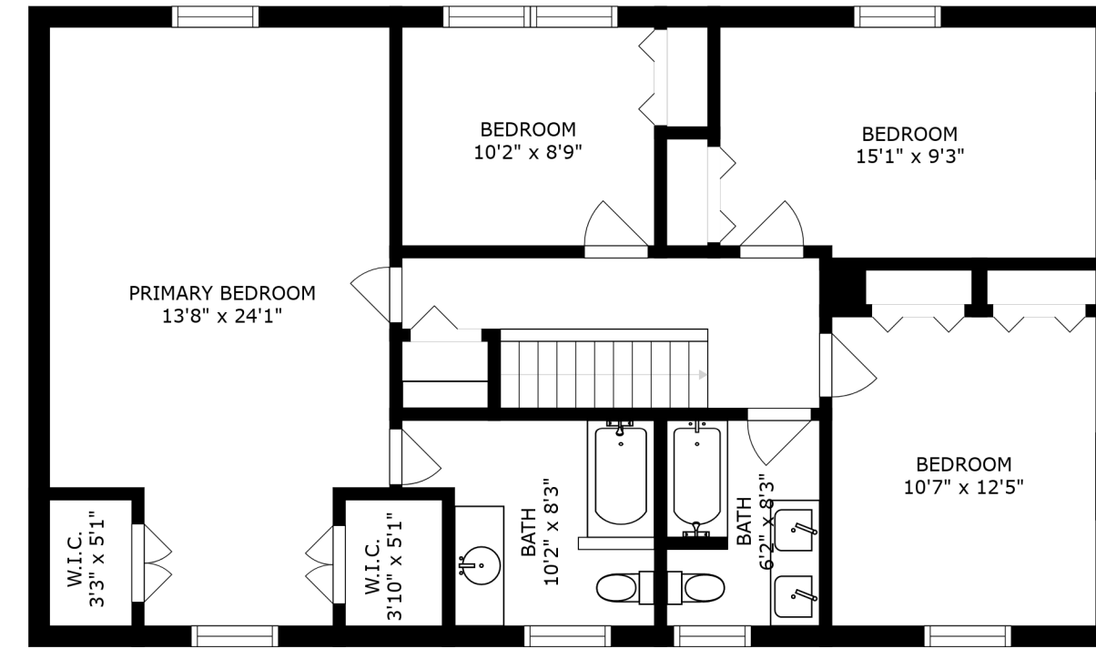
FLOOR 3
