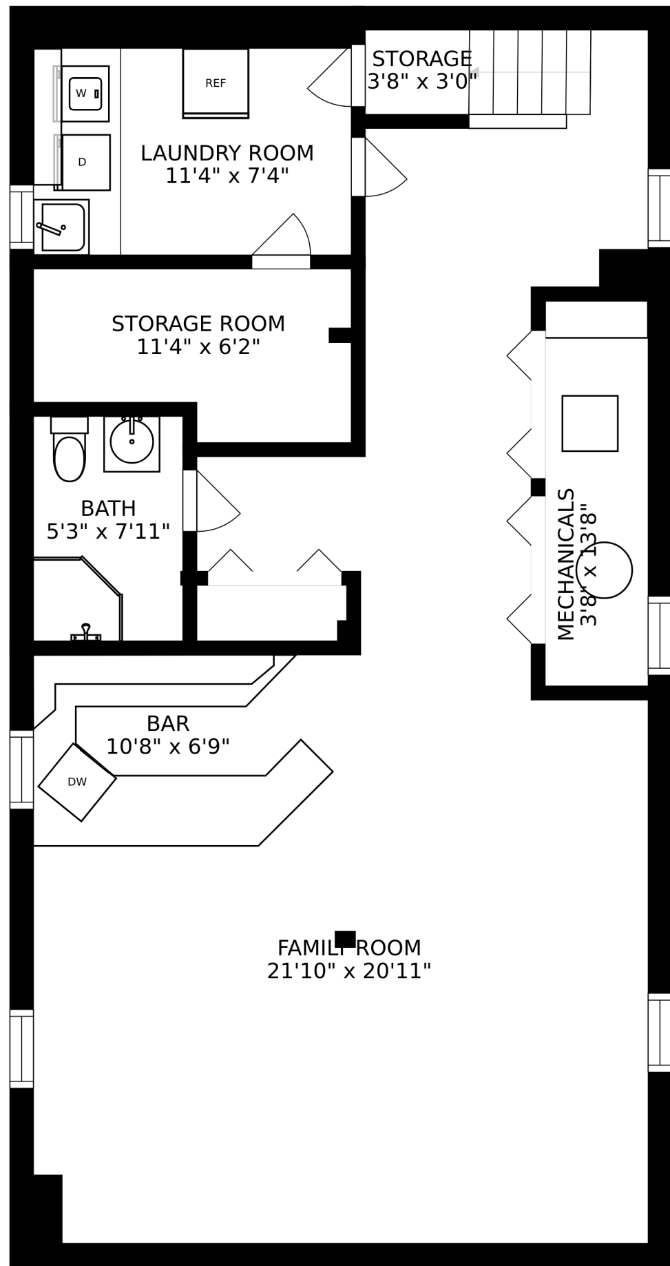
FLOOR 1
