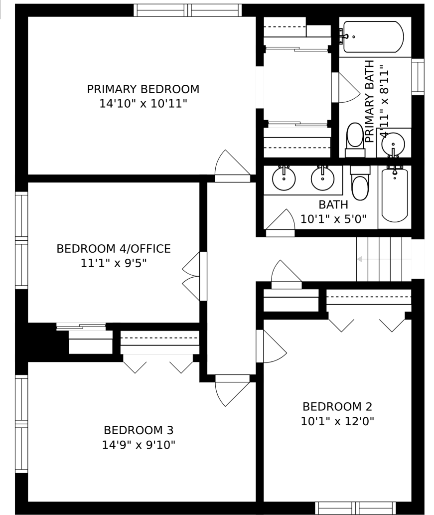
FLOOR 2
