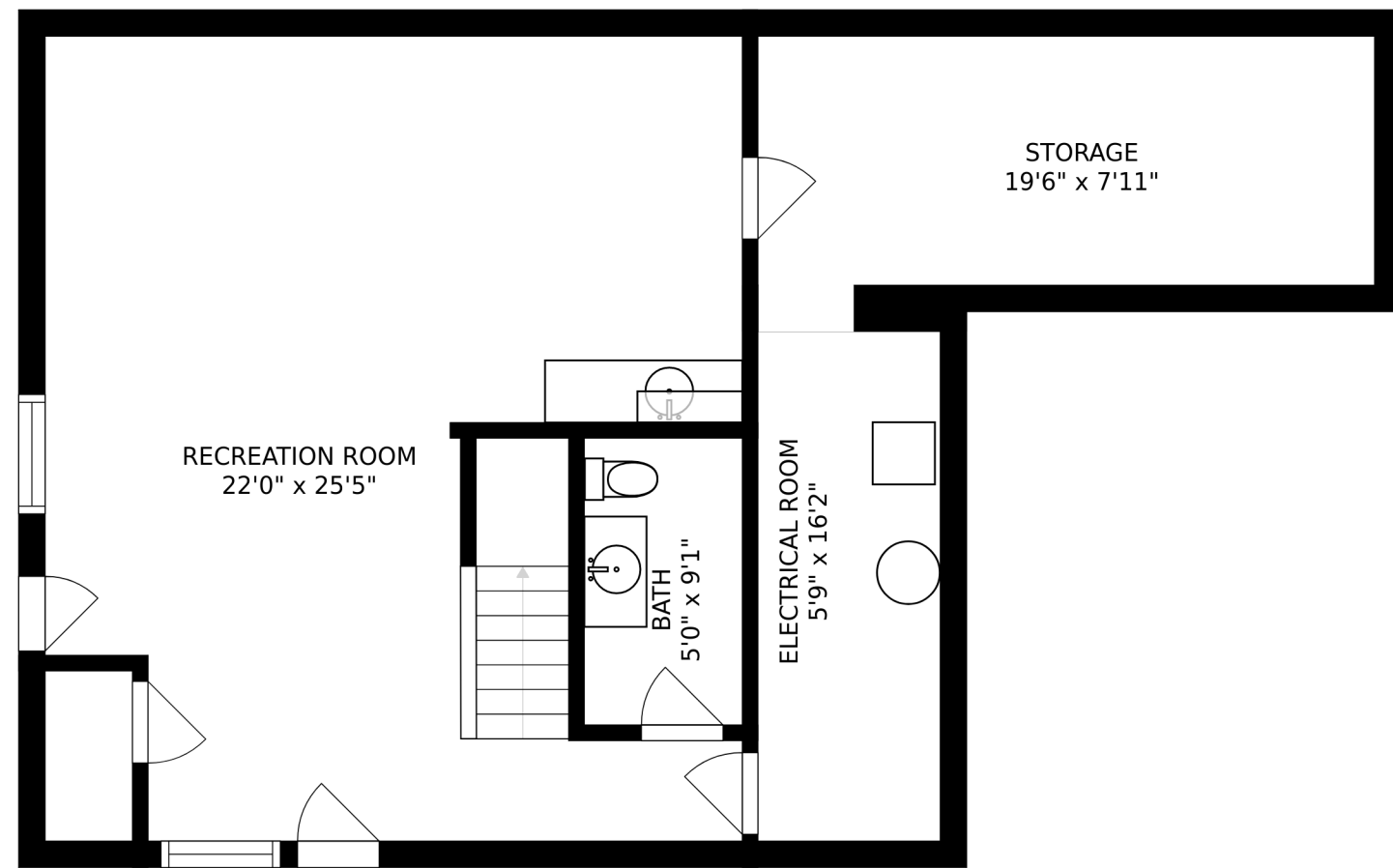
FLOOR 1
