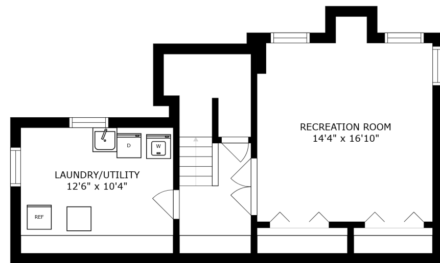
FLOOR 1
