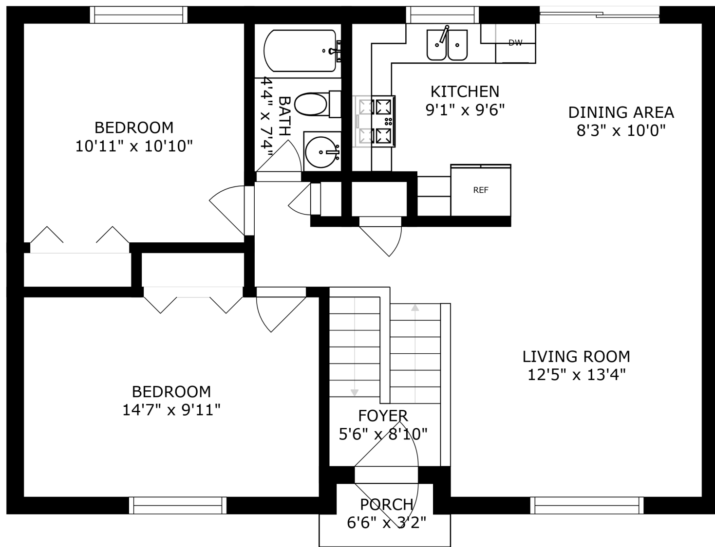
FLOOR 2
