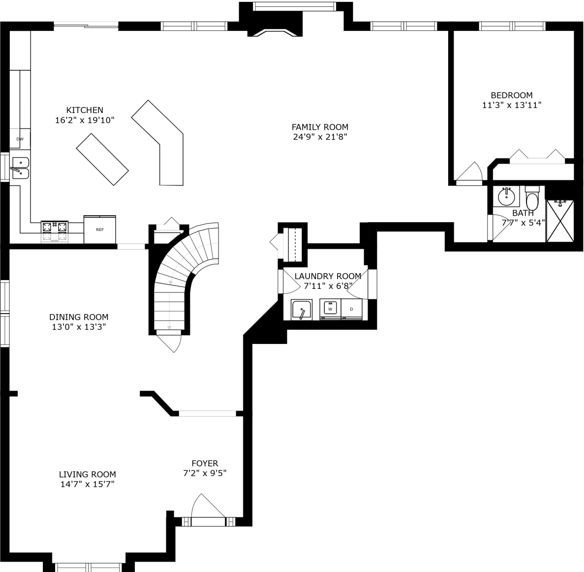
FLOOR 2
