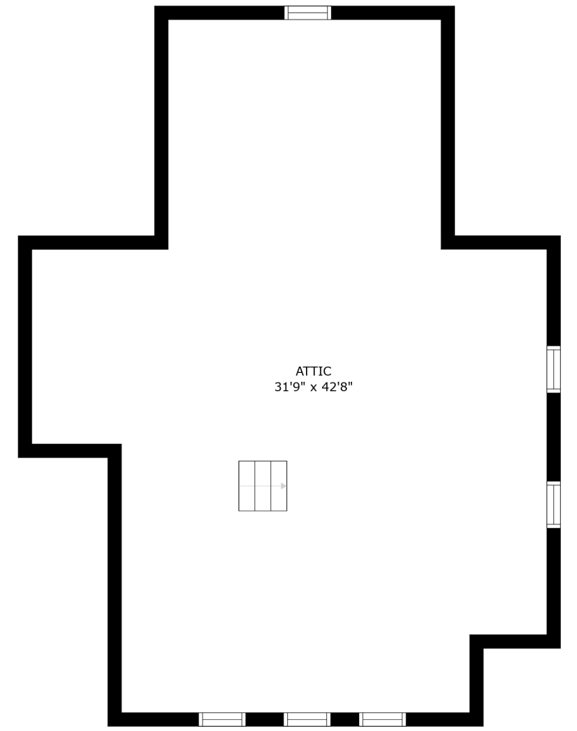
FLOOR 4
