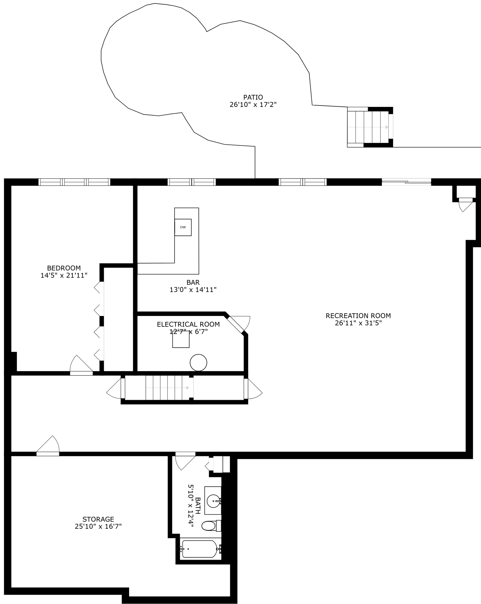
FLOOR 1
