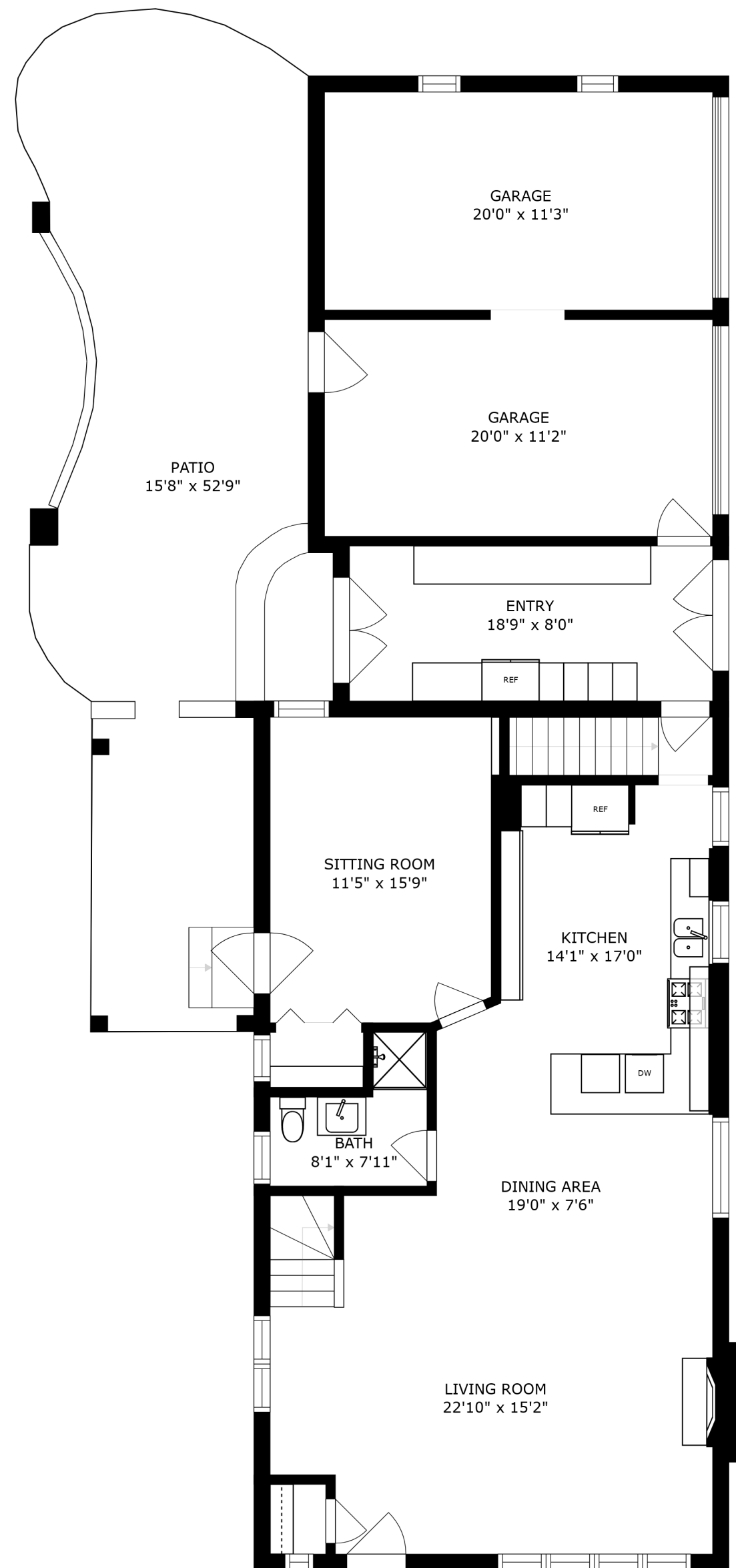
FLOOR 2
