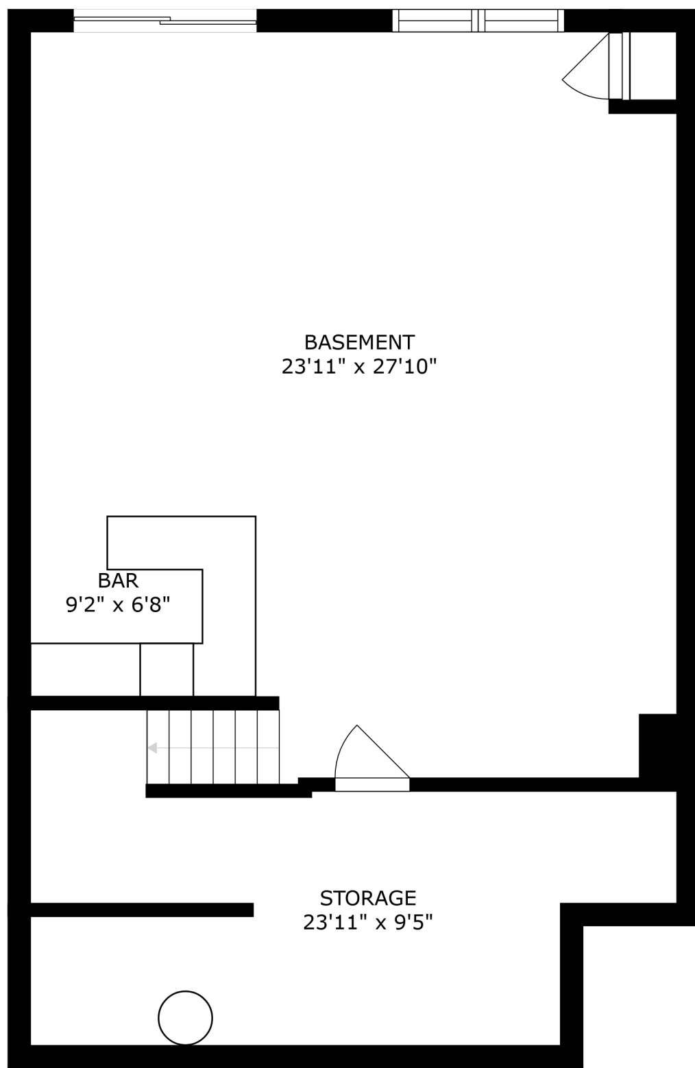
FLOOR 1
