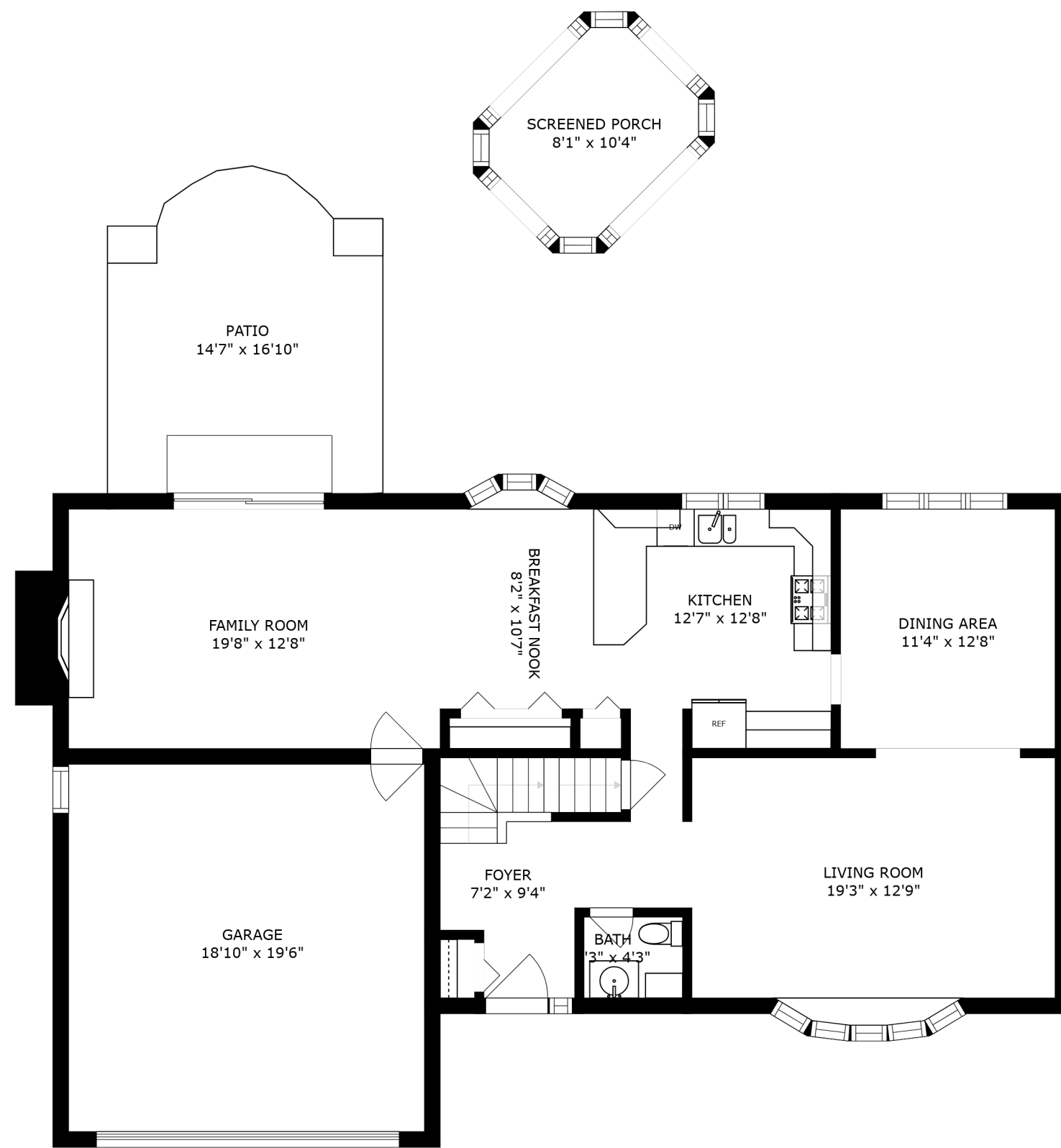
FLOOR 2
