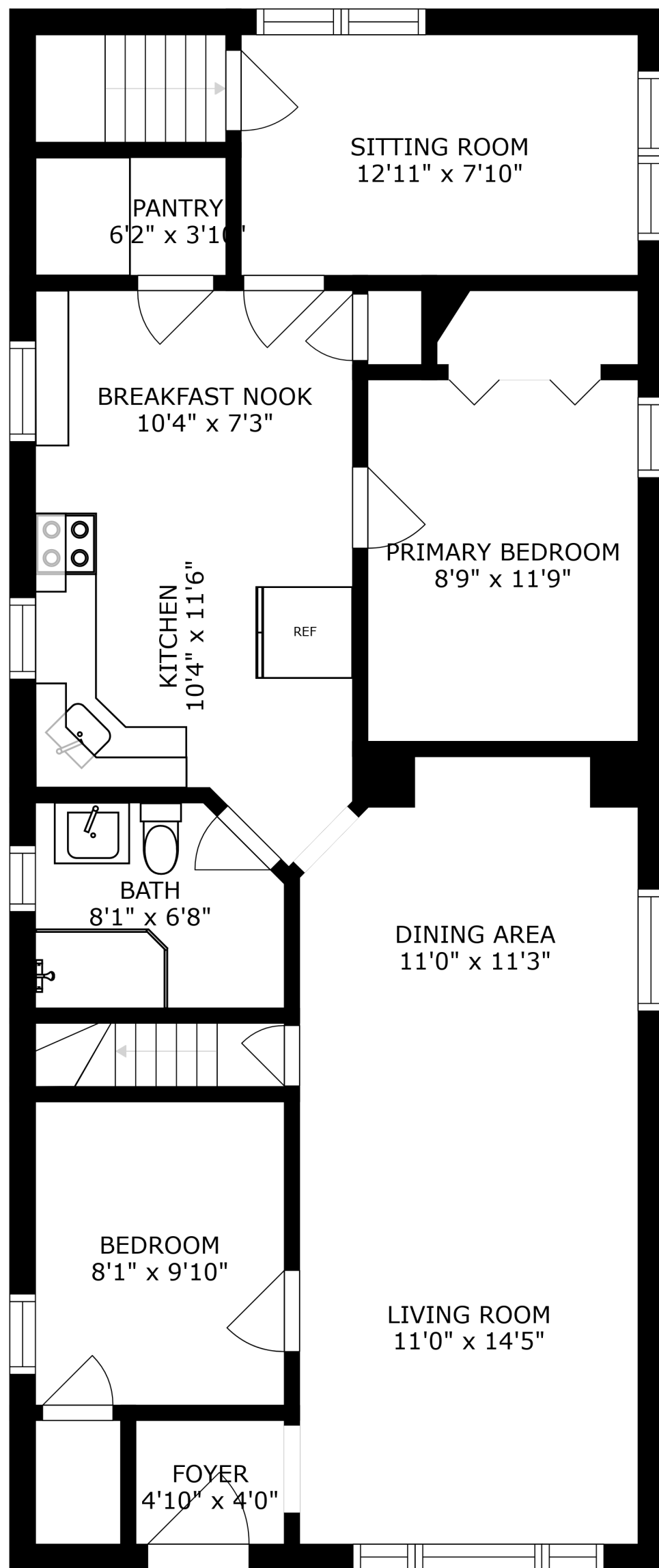
FLOOR 2
