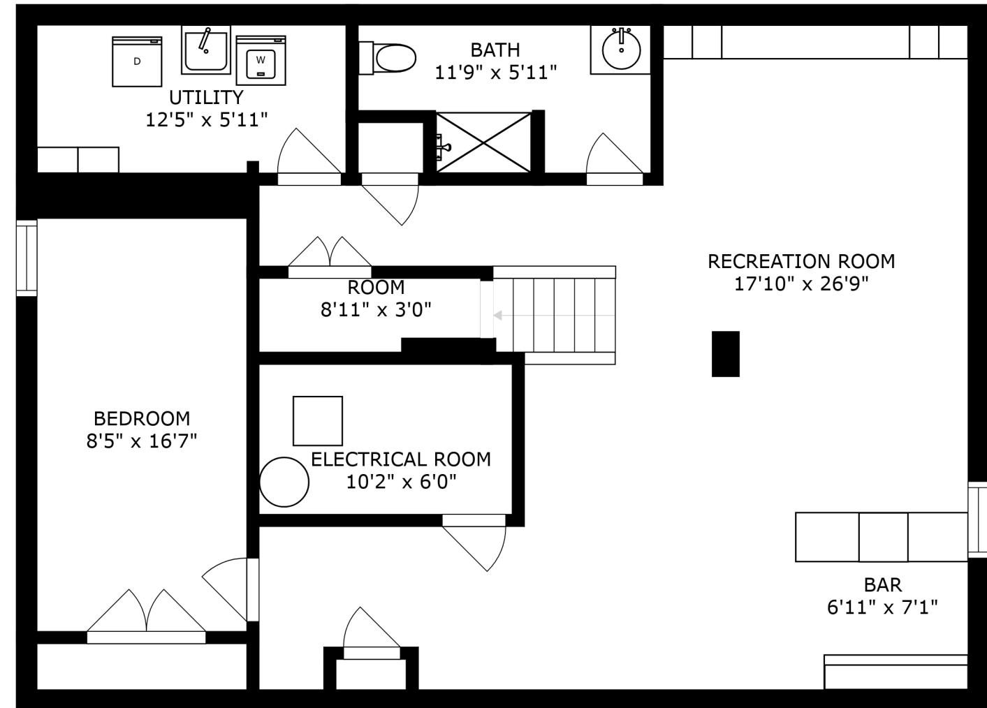
FLOOR 1
