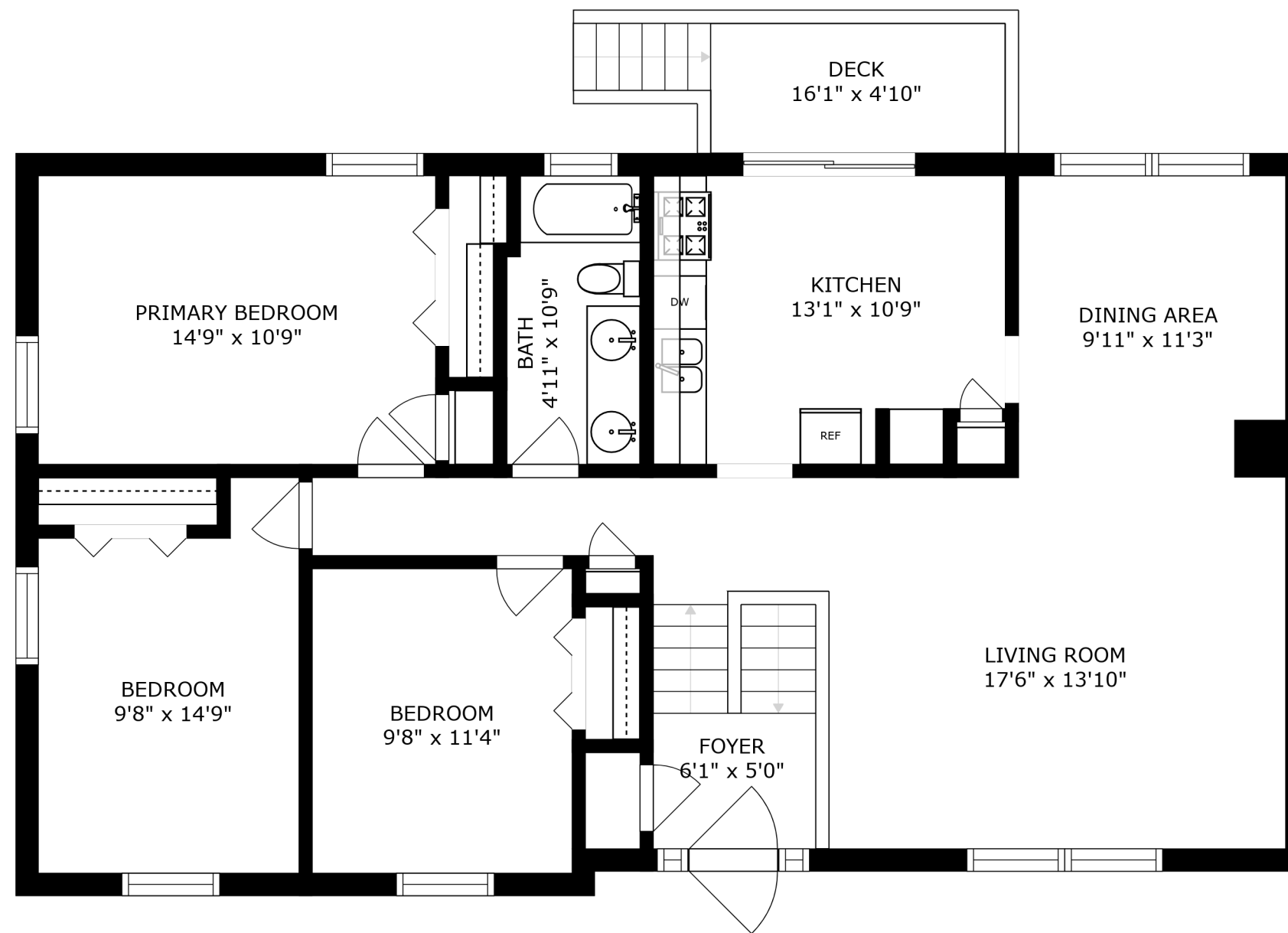
FLOOR 2
