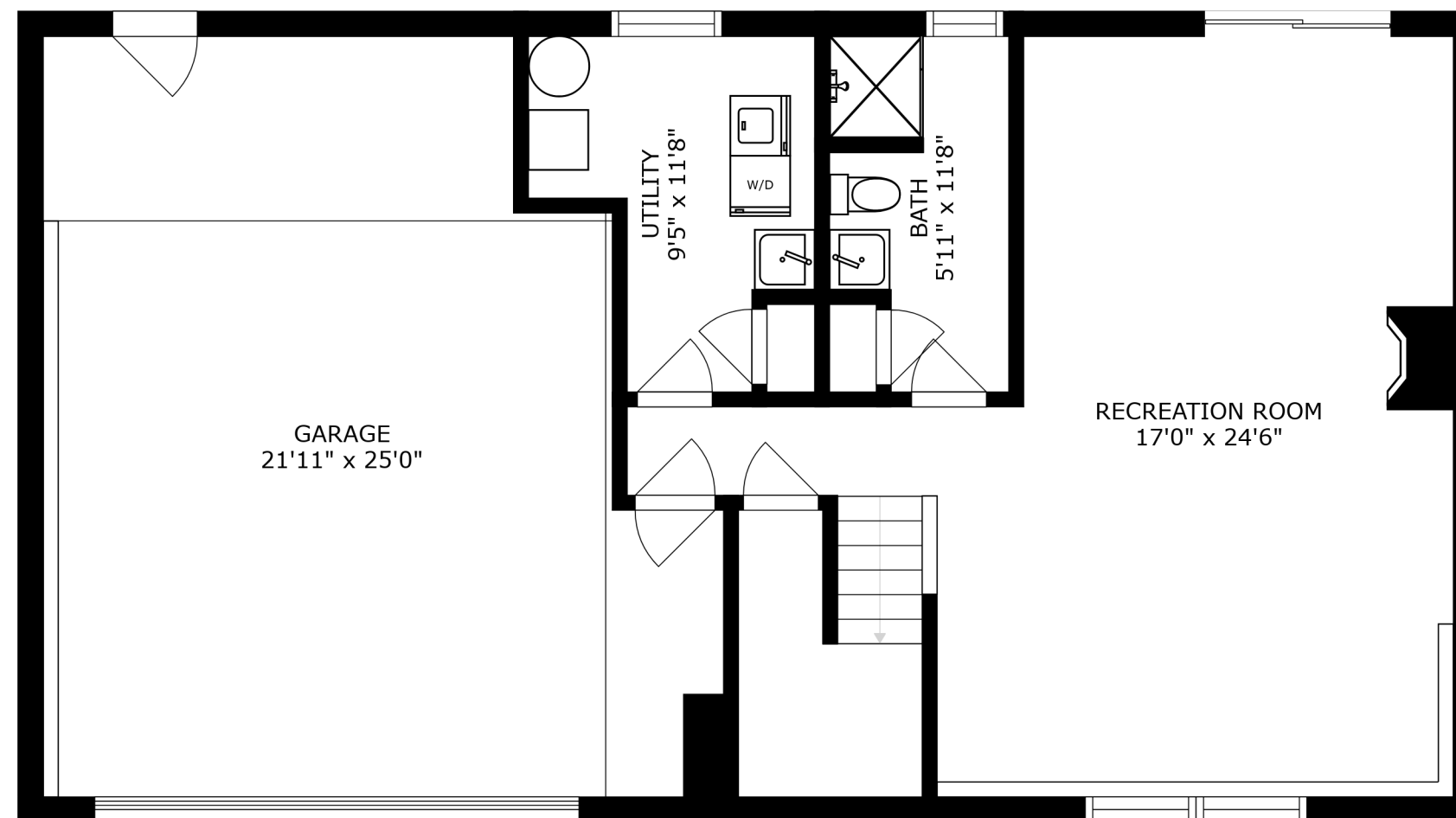
FLOOR 1
