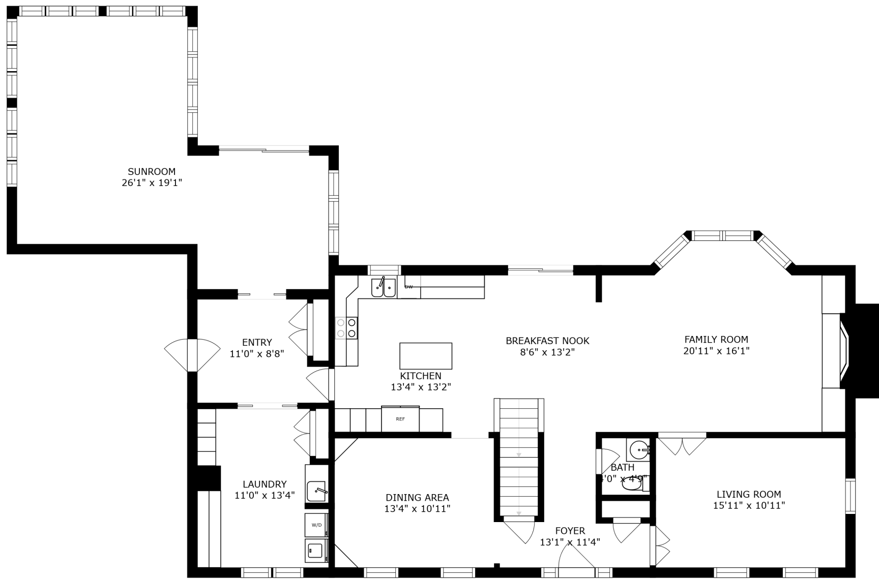
FLOOR 2
