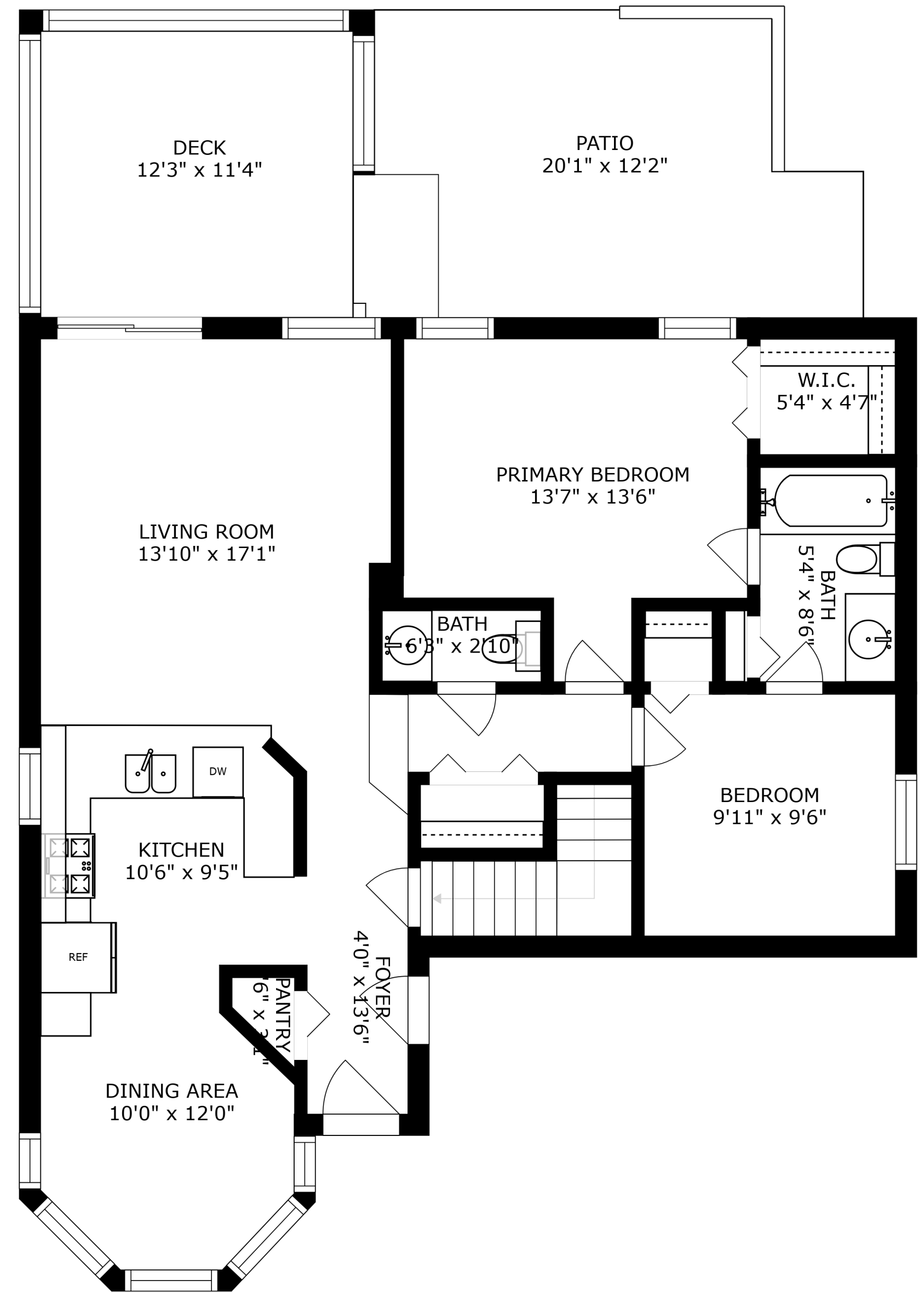
FLOOR 2
