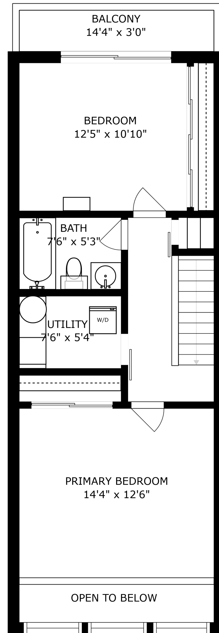
FLOOR 2
