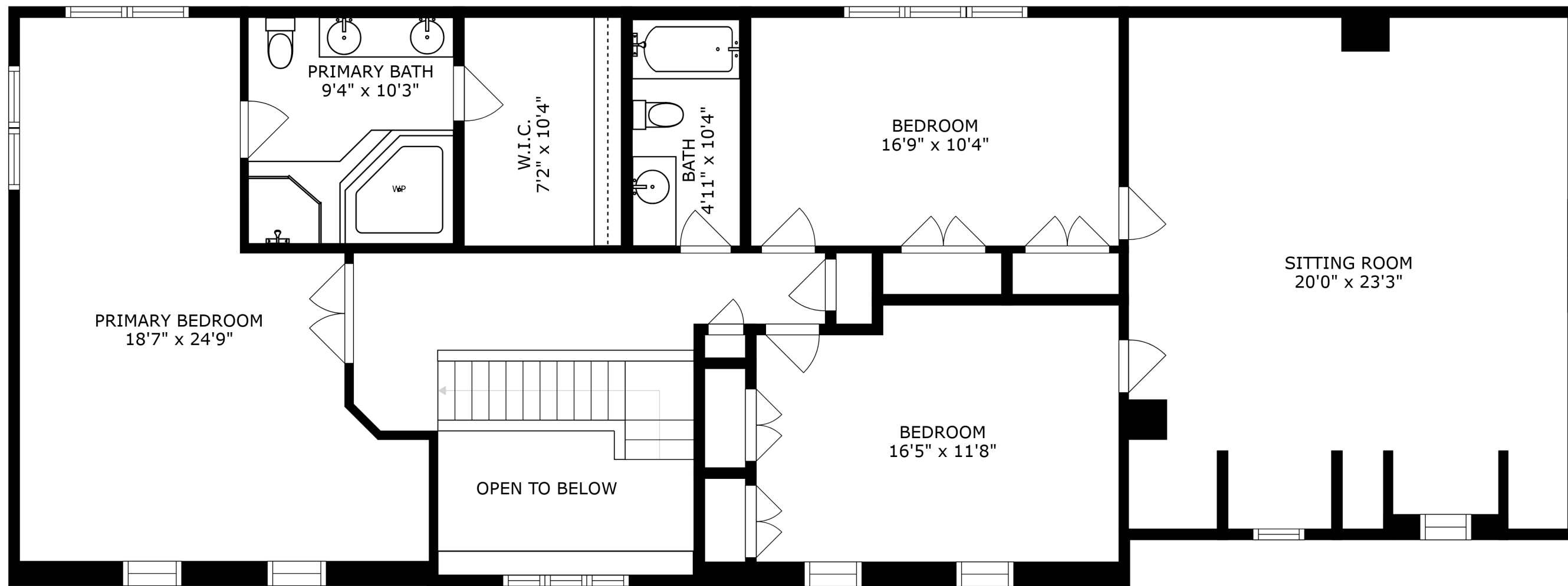
FLOOR 2
