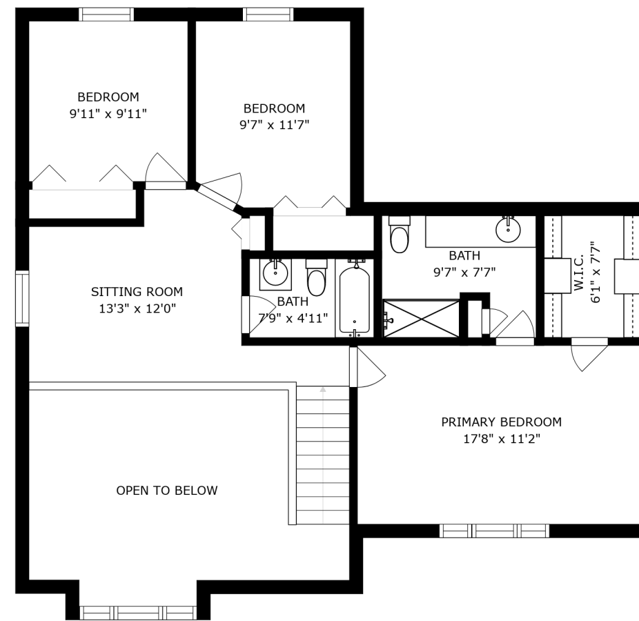
FLOOR 3
