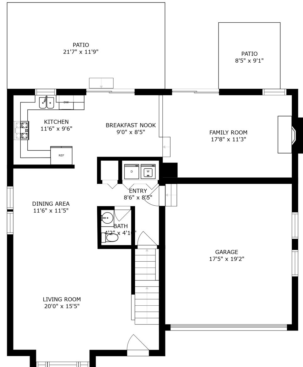
FLOOR 2
