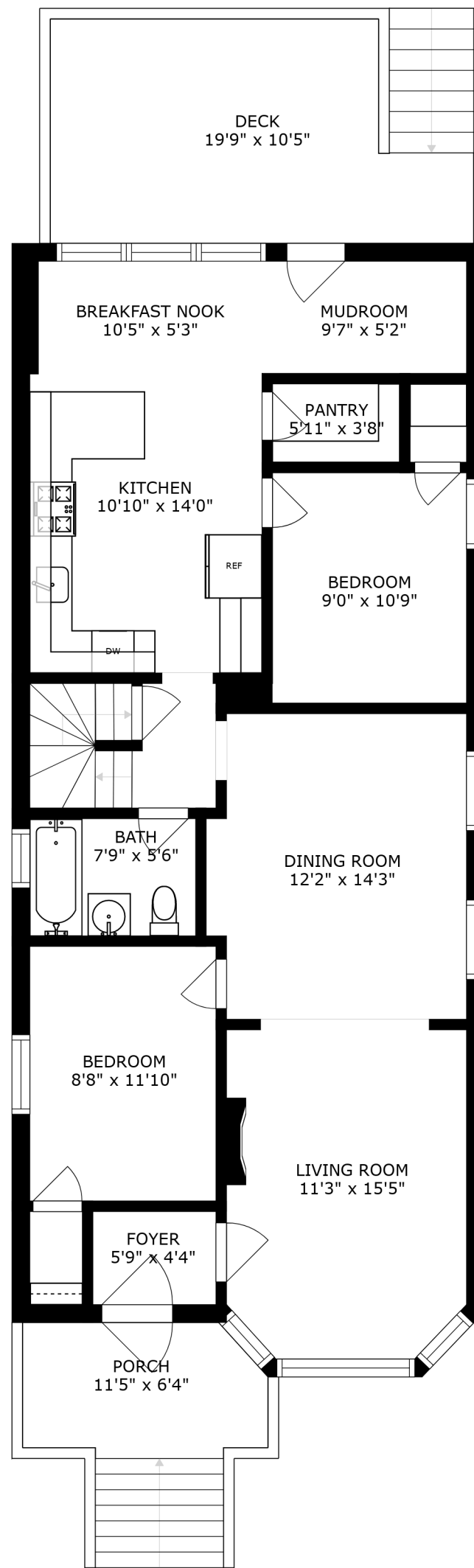
FLOOR 2
